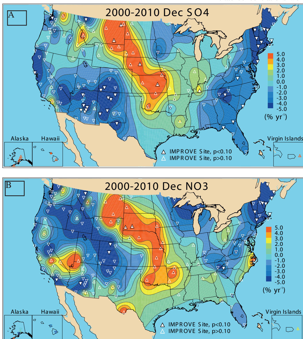
Figure 1. 2000-2010 December monthly mean trends in (A) particulate sulfate ion concentrations and (B) particulate nitrate ion concentrations. Upward and downward pointing filled triangles correspond to increasing and decreasing trends, respectively, that were significant at a 90% confidence level ( p < 0.10 ). Unfilled triangles correspond to trends with significance levels of p > 0.10 . Triangles with black dots indicate the 17 complete sites where data were used.
