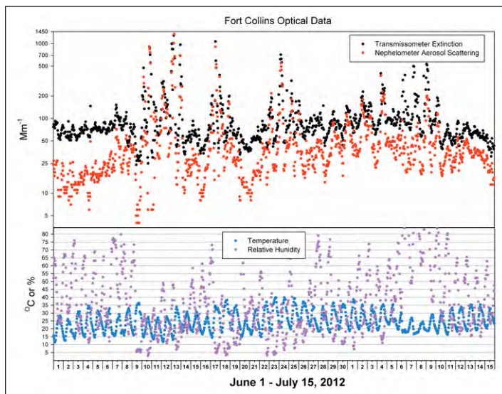
Figure 2. Fort Collins hourly optical data during Colorado fire events (note log scale for b_{ext} and b_{sp} ).
