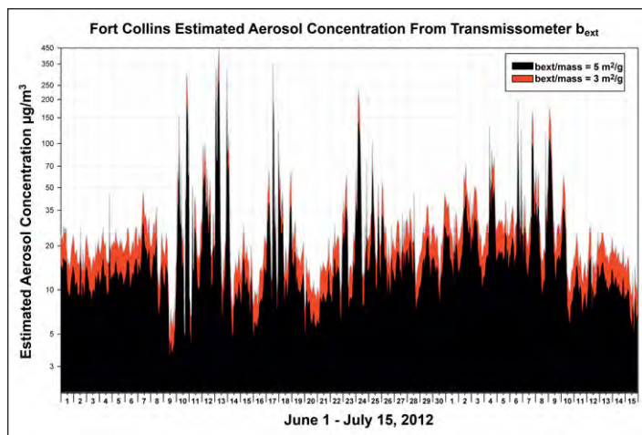
Figure 3. Aerosol concentration estimated from b_{ext} measurements.
