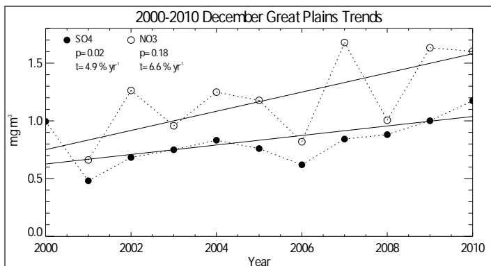
Figure 2. December monthly and regional mean concentrations ( \mu\text{g}/\text{m}^3 ) in particulate sulfate ion (filled circles) and particulate nitrate ion (open circles). Trends ( t , % \text{yr}^{-1} ) and significance levels ( p ) are provided.
