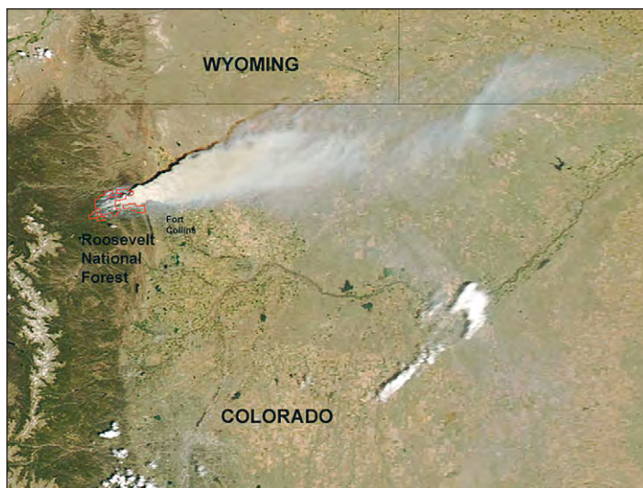
Figure 1. Satellite image of High Park Fire plume taken June 10, 2012.
