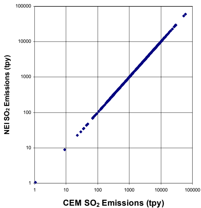
Figure 3-1. Comparison of SO 2 and NO x emissions from matched sources from the NEI 1999 and CEM 1999 databases.
