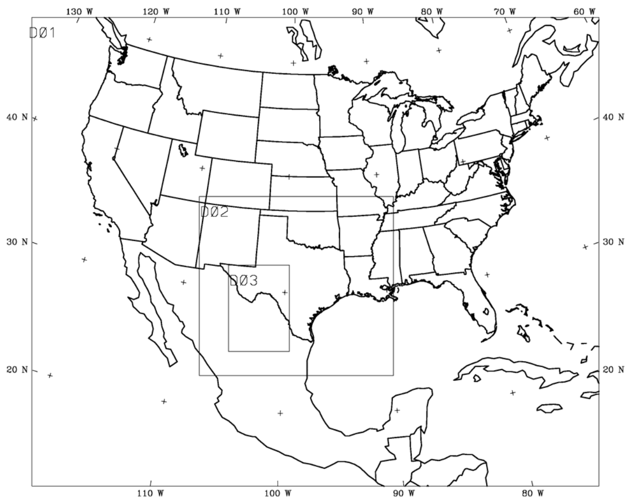
Figure 2-1. MM5 Meteorological Nested Modeling Domain.
