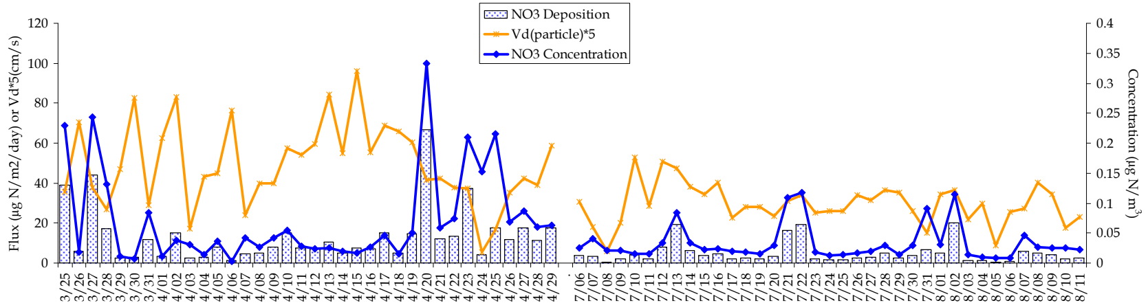
Figure 4.12. Time lines of daily deposition flux ( \mu\text{g}/\text{m}^2/\text{day} , bar), deposition velocity (cm/s, orange line), and concentration ( \mu\text{g}/\text{m}^3 , blue line) for fine particle nitrate. The deposition velocity was multiplied by a factor of 5 so all three parameters could be shown on the same plot.
