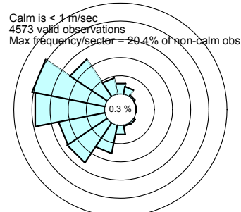
Figure 3.7. Roses showing the percent of radar profiler wind observations from each of 16 directional bins during the spring (left) and summer (right) RoMANS periods for heights of 0–1500 m (top), 1500–3000 m (second row), 3000–4500 m (third row), and 4500–6000 m (bottom) AGL. Rings are in increments of 5%.
