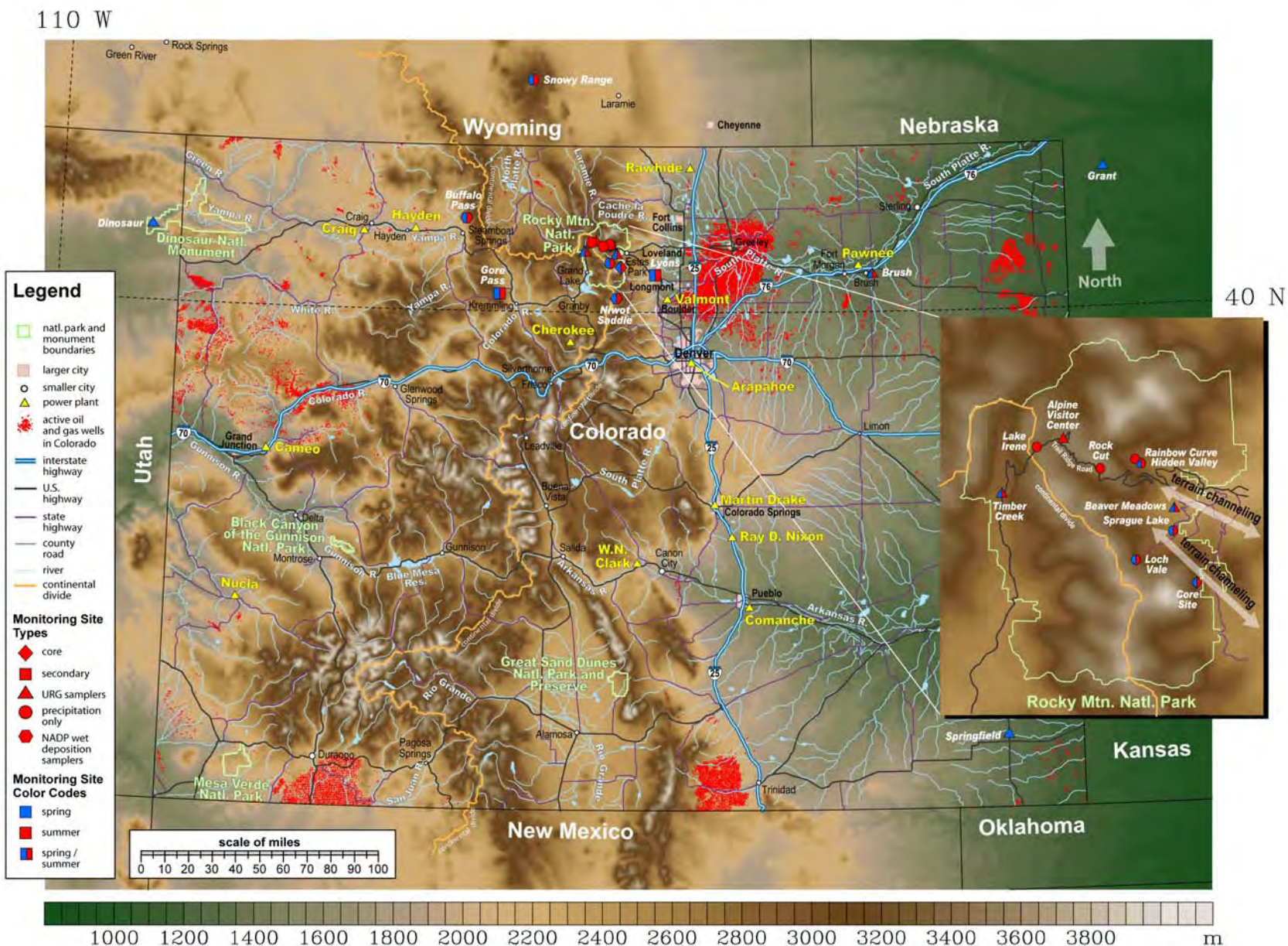
Figure 2.2. Map of Colorado and adjacent areas, illustrating the location of the monitoring sites used in the RoMANS study and the field campaign(s) during which each monitoring site was operational.
