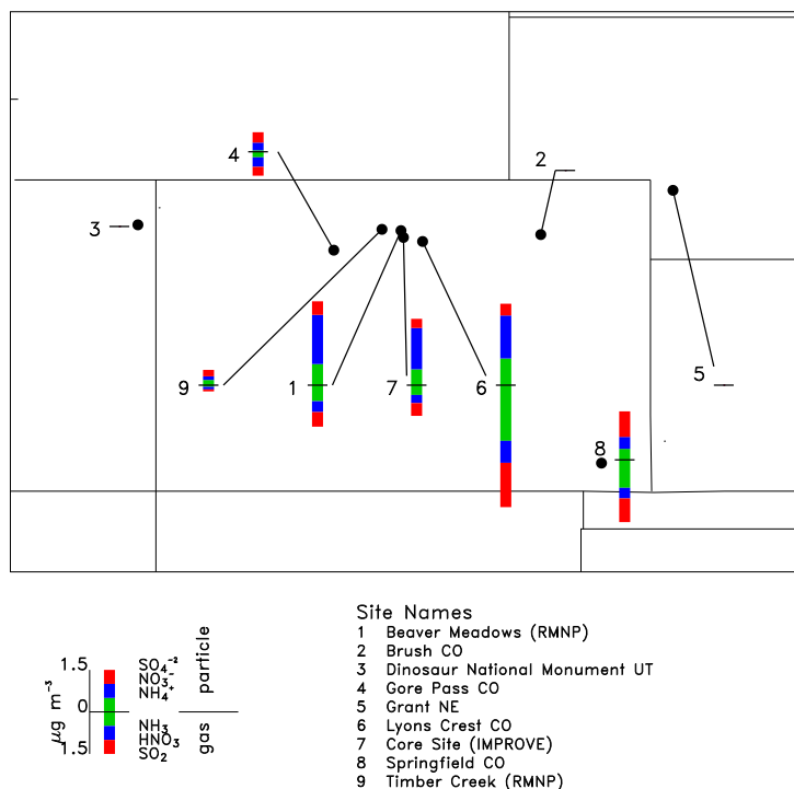
Figure 4.34. Concentrations ( \mu\text{g}/\text{m}^3 ) of oxidized and reduced fixed nitrogen species and of sulfur species measured in the RoMANS network on April 20, 2006. \text{PM}_{2.5} concentrations of nitrate, sulfate, and ammonium extend upward from the center of each bar plot; gas-phase concentrations of ammonia, nitric acid, and sulfur dioxide extend downward. Twenty-four-hr data are unavailable on this date for the Dinosaur, Brush, and Nebraska sites, which collected 48-hr samples beginning on April 19.
