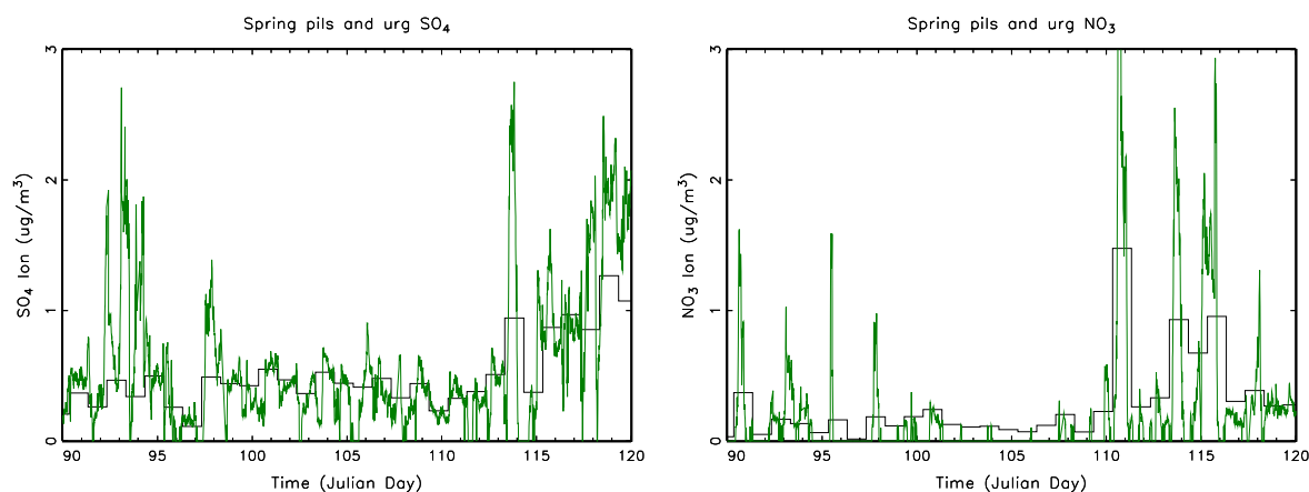
Figure S.4. Spring time series at the RoMANS core site showing (left) sulfate and (right) nitrate ion mass concentrations for the semicontinuous PILS (green) and 24-hr-average URG (black) measurement systems. Graphs are for March 31 to April 30 (Julian Days 90–120), 2006.
