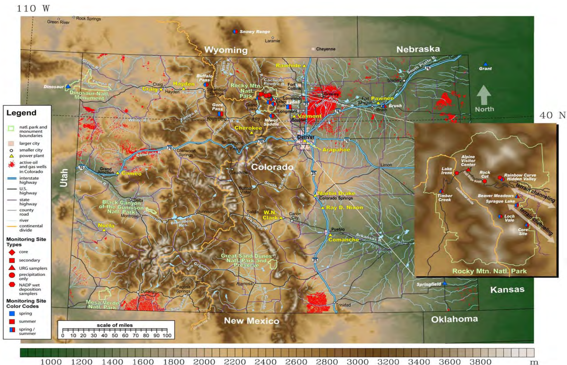
Figure S.3. Map of Colorado and adjacent areas illustrating the location of the monitoring sites used in the RoMANS study and the field campaign(s) each monitoring site was operational.
