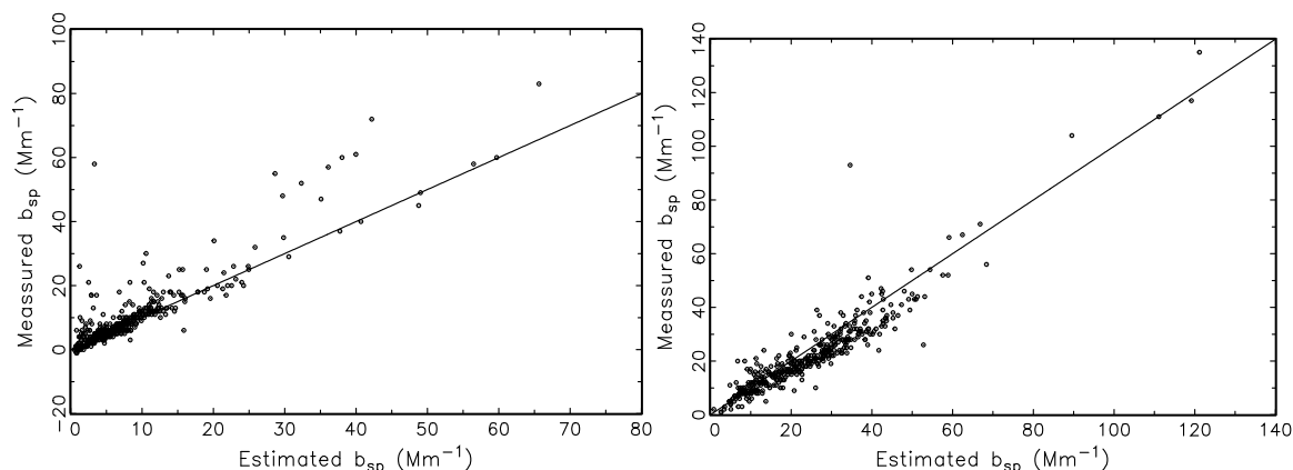
Figure 4.37. Scatter plots of reconstructed (x-axis) versus measured fine + \frac{1}{2} coarse particle scattering (y-axis) ( \text{Mm}^{-1} ) for the (left) spring and (right) summer measurement periods.
