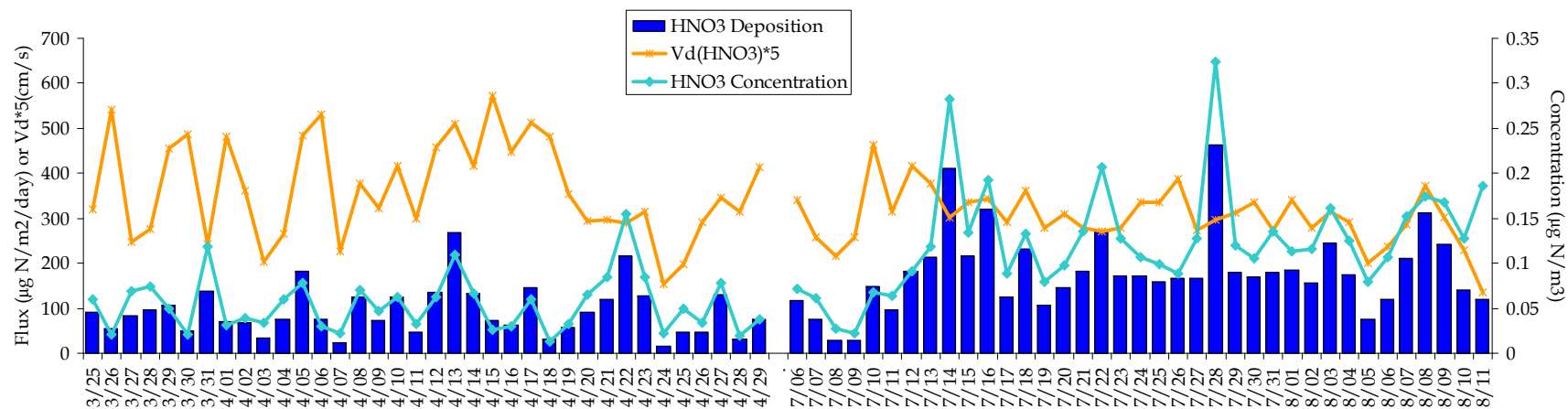
Figure 4.9. Time lines of daily deposition flux ( \mu\text{g/m}^2/\text{day} , blue bar), deposition velocity (cm/s, orange line), and concentration ( \mu\text{g/m}^3 , light blue line) for nitric acid. The deposition velocity was multiplied by a factor of 5 so all three parameters could be shown on the same plot.
