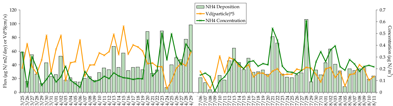
Figure 4.13. Time lines of deposition flux ( \mu\text{g/m}^2/\text{day} , bar), deposition velocity (cm/s, orange line), and concentration ( \mu\text{g/m}^3 , green line) for fine particle ammonium. The deposition velocity was multiplied by a factor of 5 so all three parameters could be shown on the same plot.
