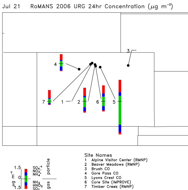
Figure 4.32. Concentrations ( \mu\text{g}/\text{m}^3 ) of oxidized and reduced fixed nitrogen species and of sulfur species measured in the RoMANS network on July 21, 2006. \text{PM}_{2.5} concentrations of nitrate, sulfate, and ammonium extend upward from the center of each bar plot; gas-phase concentrations of ammonia, nitric acid, and sulfur dioxide extend downward. Data are not available on this date for the Alpine Visitor Center or Brush sites.
