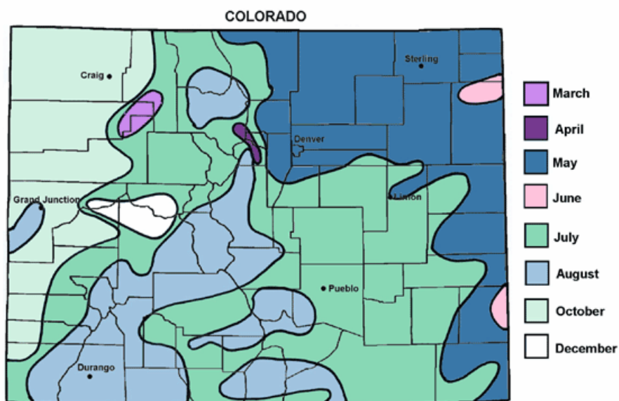
Figure 1.14. Month of maximum precipitation 1961–1990. Downloaded from http://ccc.atmos.colostate.edu/wettestmonth.php .
