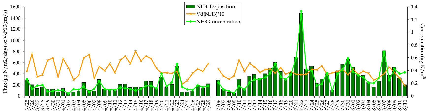
Figure 4.10. Time lines of daily deposition flux ( \mu\text{g/m}^2/\text{day} , green bar), deposition velocity (cm/s, orange line), and concentration ( \mu\text{g/m}^3 , light green line) for ammonia. The deposition velocity was multiplied by a factor of 10 so all three parameters could be shown on the same plot.
