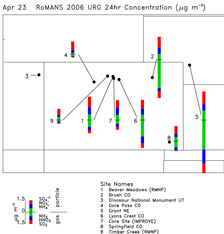
Figure 4.35. Concentrations ( \mu\text{g}/\text{m}^3 ) of oxidized and reduced fixed nitrogen species and of sulfur species measured in the RoMANS network on April 23, 2006. \text{PM}_{2.5} concentrations of nitrate, sulfate, and ammonium extend upward from the center of each bar plot; gas-phase concentrations of ammonia, nitric acid, and sulfur dioxide extend downward. Twenty-four-hr data are unavailable on this date for the Dinosaur site.
