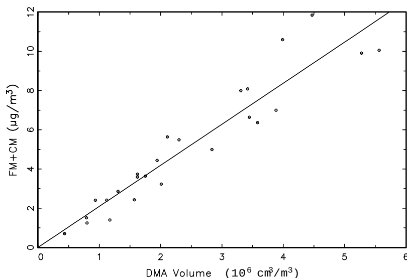
Figure 3.38. An example scatter plot of 24-hr-average PM_{10} mass concentrations ( \mu\text{g}/\text{m}^3 ) (y-axis) versus total particle volume concentration as derived from the particle number size distributions.
