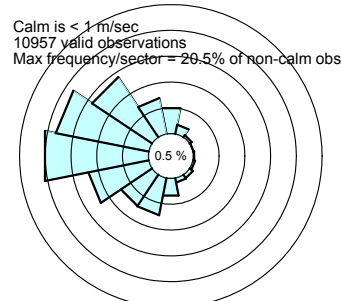
Estes Park Radar Profiler summer 97-m mode 4500-6000 m AGL
