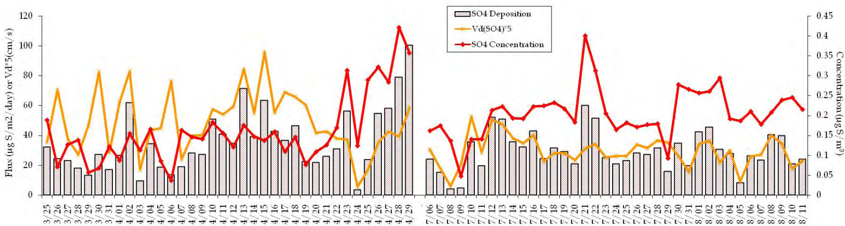
Figure 4.14. Time lines of deposition flux ( \mu\text{g/m}^2/\text{day} , bar), deposition velocity (cm/s, orange line), and concentration ( \mu\text{g/m}^3 , red line) for fine particle sulfate. The deposition velocity was multiplied by a factor of 5 so all three parameters could be shown on the same plot.
