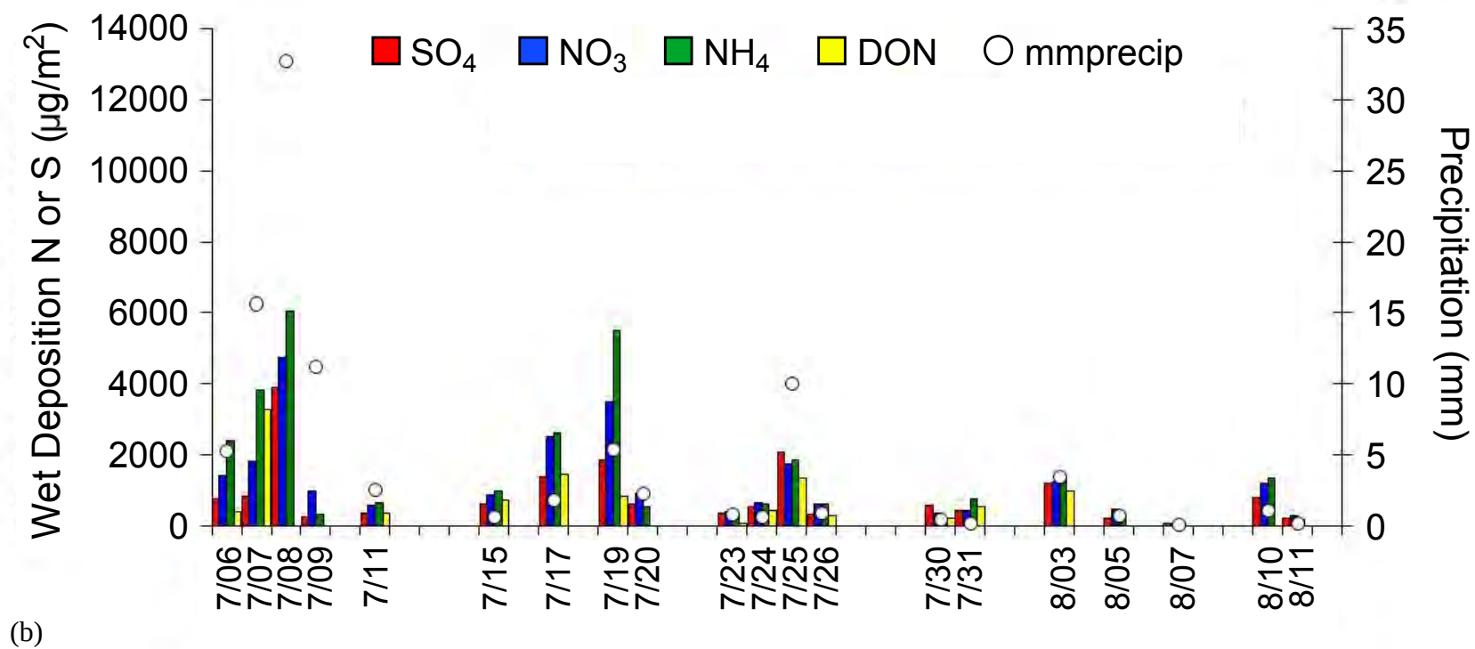
Figure 3.11. Time line of daily wet deposition fluxes ( \mu\text{g}/\text{m}^2 ) of major nitrogen and sulfur species at the RoMANS core site during the (a) spring and (b) summer field campaigns.
