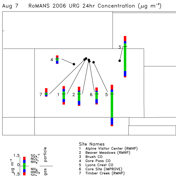
Figure 4.33. Concentrations ( \mu\text{g}/\text{m}^3 ) of oxidized and reduced fixed nitrogen species and of sulfur species measured in the RoMANS network on August 7, 2006. \text{PM}_{2.5} concentrations of nitrate, sulfate, and ammonium extend upward from the center of each bar plot; gas-phase concentrations of ammonia, nitric acid, and sulfur dioxide extend downward.
