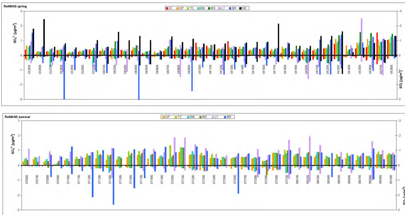
Figure 4.28. Daily concentrations ( \mu\text{g}/\text{m}^3 ) of sulfate and sulfur dioxide measured at selected RoMANS network sites during the spring (top panel) and summer (bottom panel) campaigns. Sites are arranged from west to east. PM 2.5 sulfate concentrations are represented by bars extending upward from the center of each plot; sulfur dioxide concentrations are represented by bars extending downward (right axis).
