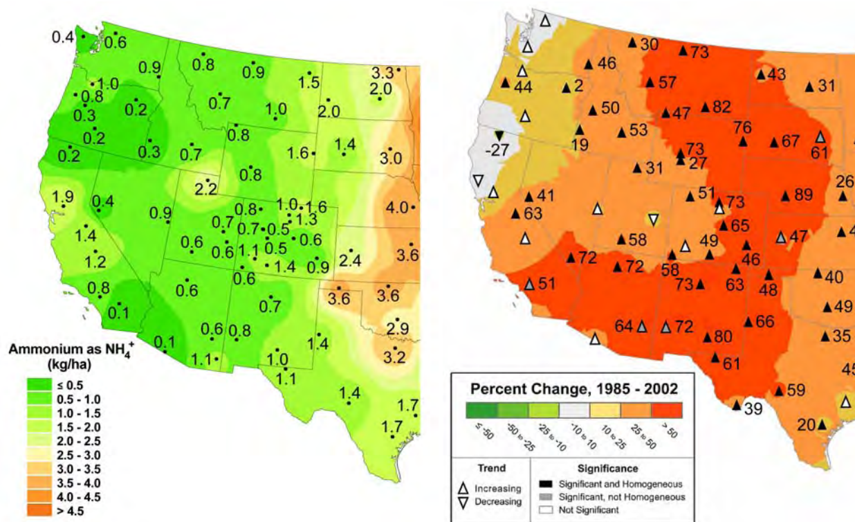
Figure 1.9. Left panel: Ammonium ion annual wet deposition for 2002 in kg/ha (Source: National Acid Deposition Program/National Trends Network). Right panel: Percent changes in the ammonium concentrations in precipitation for the years 1985–2002 (Lehmann et al., 2005, reproduced without permission).
