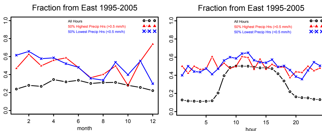
Figure 1.11. Fractions of winds from the east by month and by hour of day for 1995–2005. Fractions are shown for all hours and for hours with light precipitation and heavy precipitation. Data are from the NPS gaseous monitoring network 10-m tower at RMNP.
