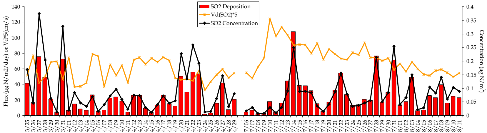
Figure 4.11. Time lines of daily deposition flux ( \mu\text{g}/\text{m}^2/\text{day} , red bar), deposition velocity (cm/s, orange line), and concentration ( \mu\text{g}/\text{m}^3 , black line) for sulfur dioxide. The deposition velocity was multiplied by a factor of 5 so all three parameters could be shown on the same plot.
