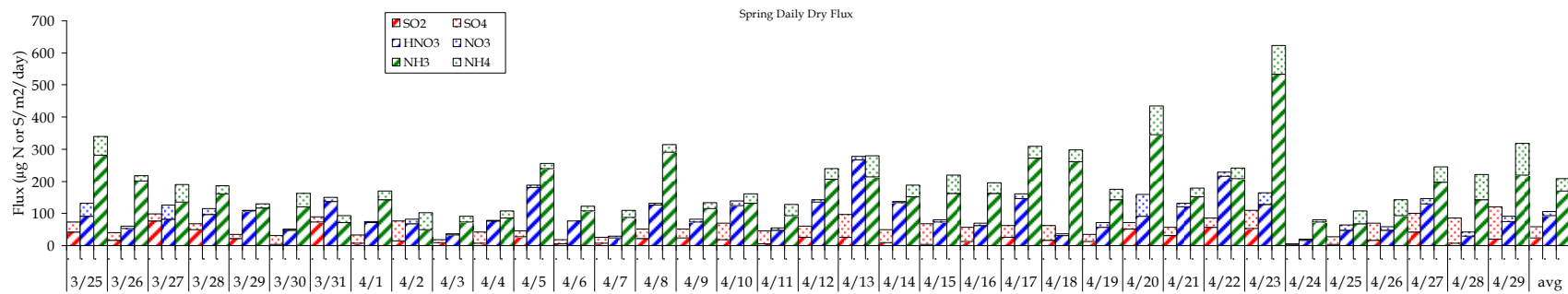
Figure 4.7. Spring dry daily deposition ( \mu\text{g}/\text{m}^2/\text{day} ) of reduced and oxidized nitrogen and of sulfur at the RoMANS core site. Particle fluxes are shown in the dotted bars and gas fluxes are shown in the hatched bars. Red: \text{SO}_4^{2-}/\text{SO}_2 , blue: \text{NO}_3^-/\text{HNO}_3 , and green: \text{NH}_4^+/\text{NH}_3 .
