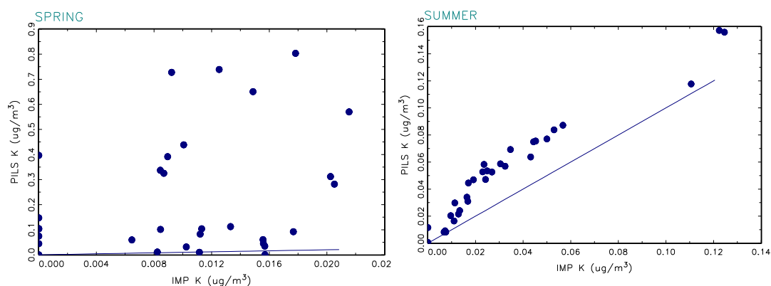
Figure 3.31. PM 2.5 potassium concentration (µg/m 3 ) comparisons from PILS (24-hr average) on the y-axis and IMPROVE on the x-axis for spring (left) and summer (right). The 1:1 line is shown for reference.
