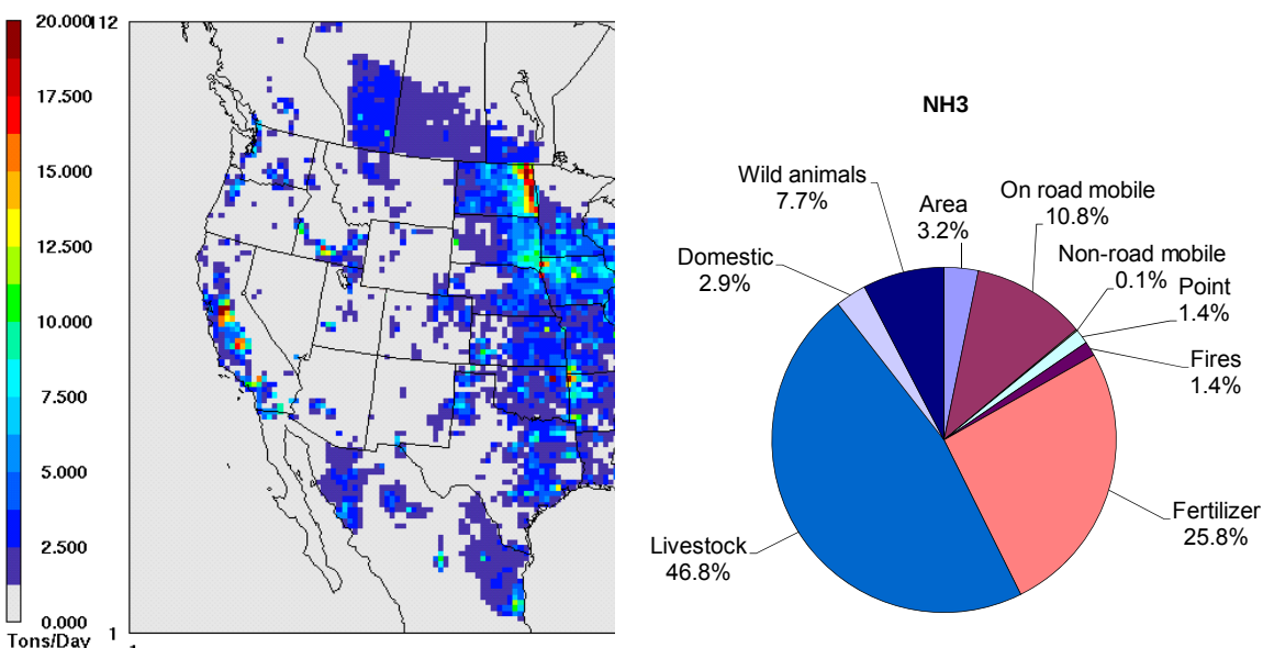
Figure S.9. Spatial distribution of annual average emissions of (top) \text{NO}_x and (bottom) \text{NH}_3 . The pie charts show the contribution of different emission types within Colorado to \text{NO}_x and \text{NH}_3 .
