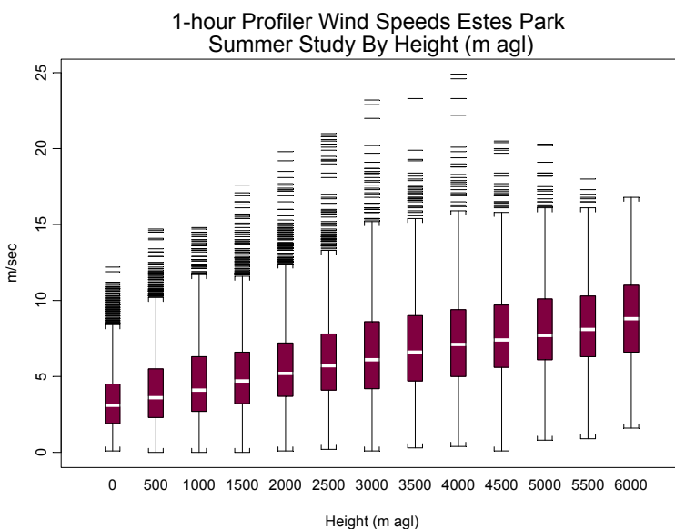
Figure 3.9. Box plots of radar wind profiler wind speeds (m/sec) by height during the summer RoMANS study.
