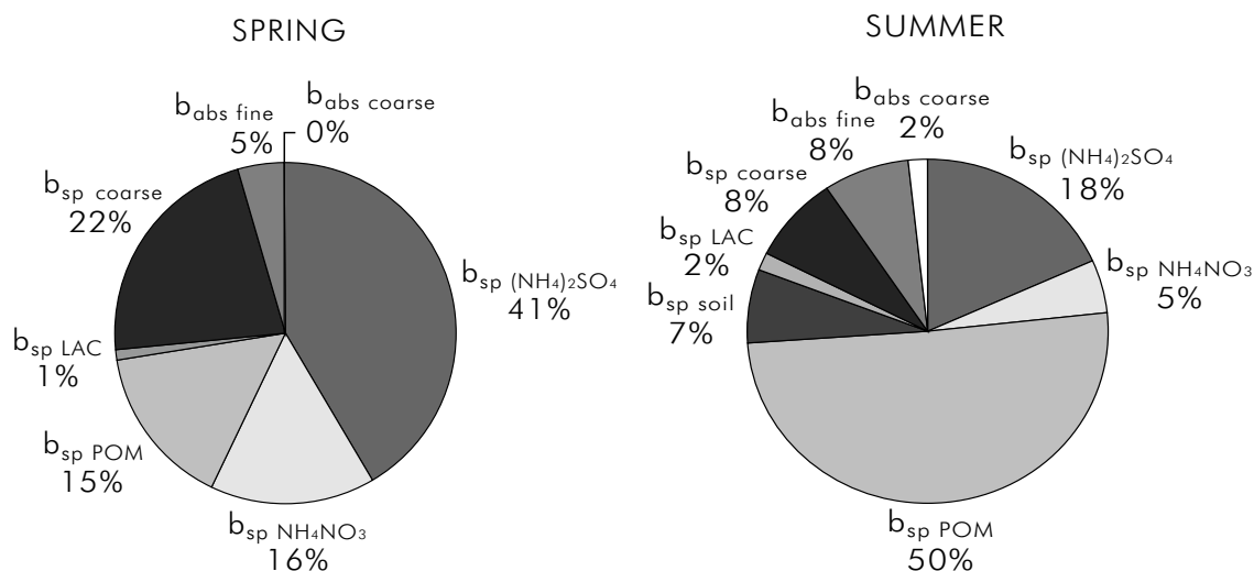
Figure 4.38. Approximate extinction budgets for the (left) spring and (right) summer time periods.
