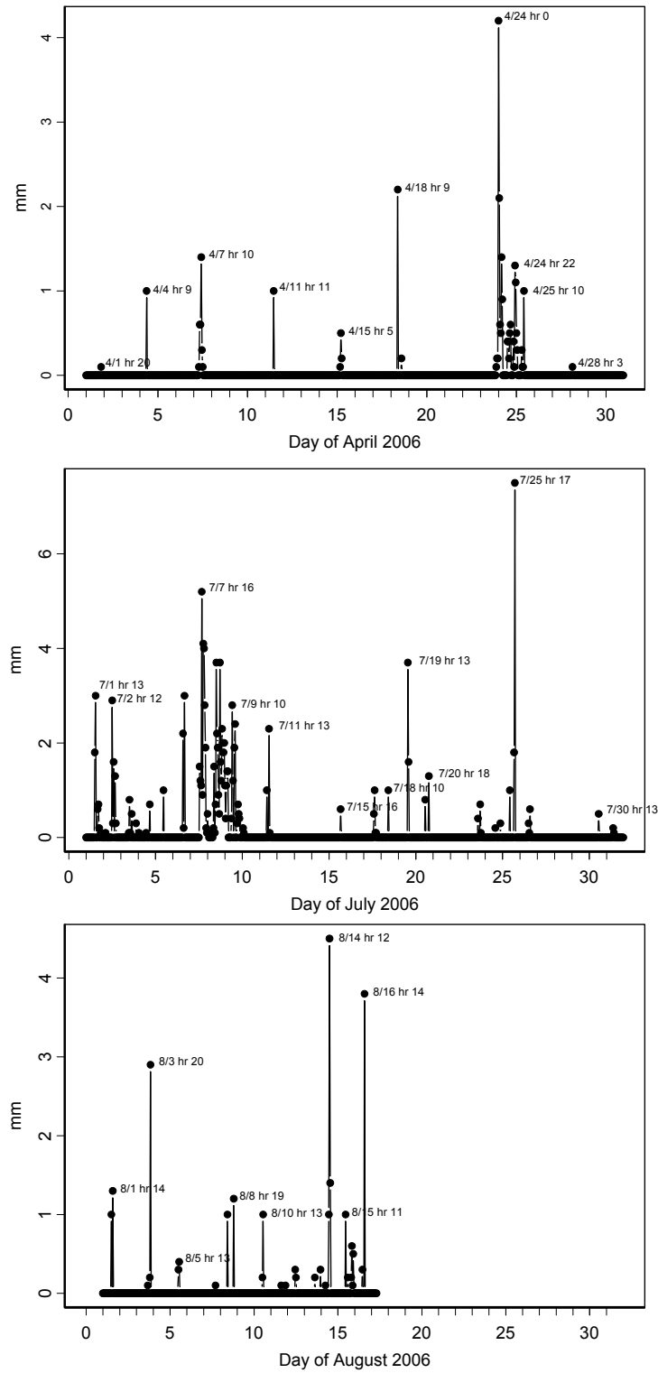
Figure 3.1. Hourly precipitation (mm) measured at the RoMANS core site during April (top), July (middle), and August (bottom) of 2006.
