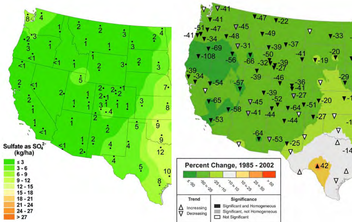
Figure 1.7. Left panel: Sulfate ion 2002 annual wet deposition rates in kg/ha (Source: National Acid Deposition Program/National Trends Network). Right panel: Percent changes in the sulfate concentrations in precipitation for the years 1985–2002 (Lehmann et al., 2005, reproduced without permission).
