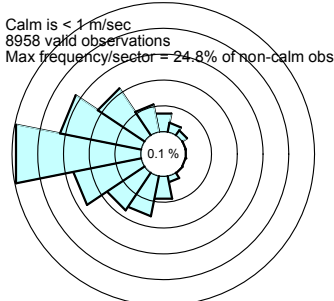
Estes Park Radar Profiler spring 97-m mode 3000-4500 m AGL
