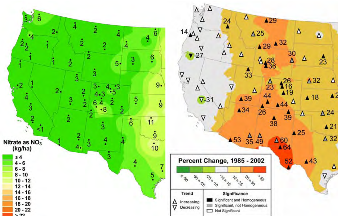
Figure 1.8. Left panel: Nitrate ion 2002 annual wet deposition in kg/ha (Source: National Acid Deposition Program/National Trends Network). Right panel: Percent changes in the nitrate concentrations in precipitation for the years 1985–2002 (Lehmann et al., 2005, reproduced without permission).
