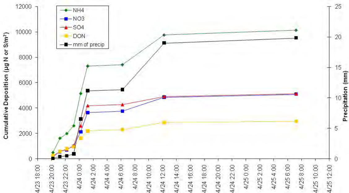
Figure 3.13. Time evolution of cumulative precipitation (mm) and wet deposition ( \mu\text{g}/\text{m}^2 ) of major solute species at the RoMANS core site during the period April 23 through April 25, 2006.
