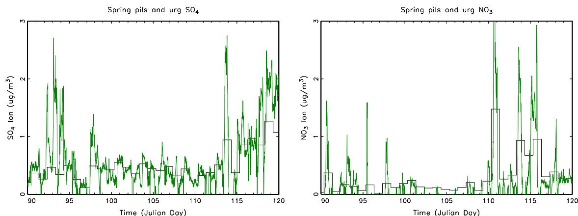
Figure 3.27. Graphs of spring time series showing (left) sulfate and (right) nitrate ion mass concentrations ( \mu\text{g}/\text{m}^3 ) for the semicontinuous PILS (green) and 24-hr-average URG measurement systems.
