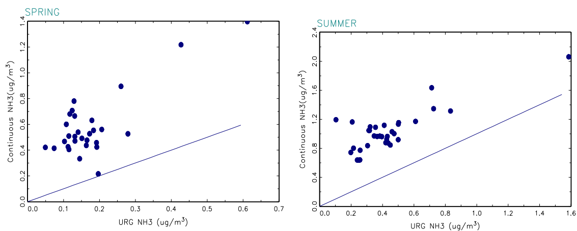
Figure 3.32. Ammonia concentration (µg/m 3 ) comparisons from continuous gas measurements (24-hr average) on the y-axis and URG on the x-axis for spring (left) and summer (right). The 1:1 line is shown for reference.
