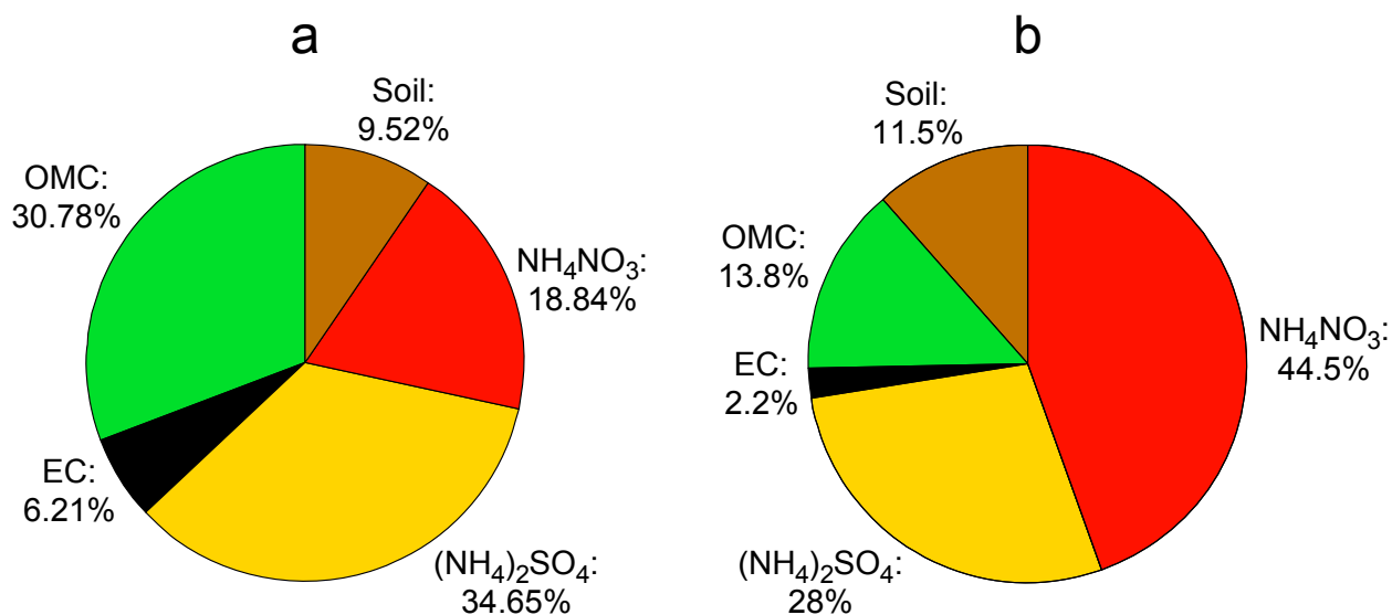
Figure 1.4. (a) Twelve-year-average winter fine particle mass composition in RMNP. (b) RMNP fine mass composition on March 3, 2002. Species included are ammonium nitrate, ammonium sulfate, elemental carbon (EC), organic matter (OMC), and fine particle soil.
