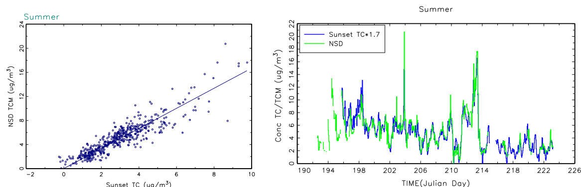
Figure 3.40. Scatter plot (left) of total carbon (TC = POM + LAC) as measured by the Sunset carbon analyzer (x-axis) and total carbon mass (TCM) derived from total number size distributions (y-axis). Time series (right) of Sunset total carbon (blue) and total carbon derived from size distributions (green). Units of \mu\text{g}/\text{m}^3 .
