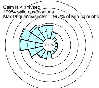
Estes Park Radar Profiler summer 97-m mode 3000-4500 m AGL
