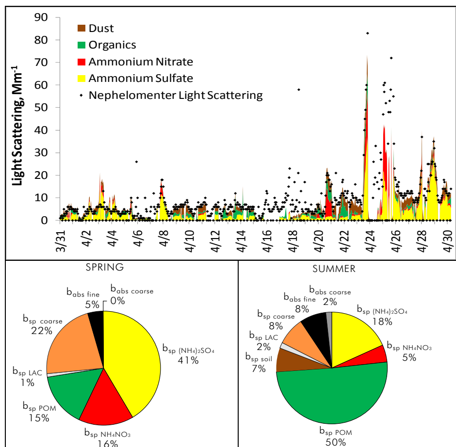
Figure S.6. Temporal plot of measured and estimated particulate atmospheric scattering ( \text{Mm}^{-1} ) of major aerosol species at the core monitoring site during the spring RoMANS time period and the approximate extinction budgets for the spring and summer RoMANS time periods. Note, gaps in the extinction budgets, e.g., April 16–17, are due to missing aerosol data.
