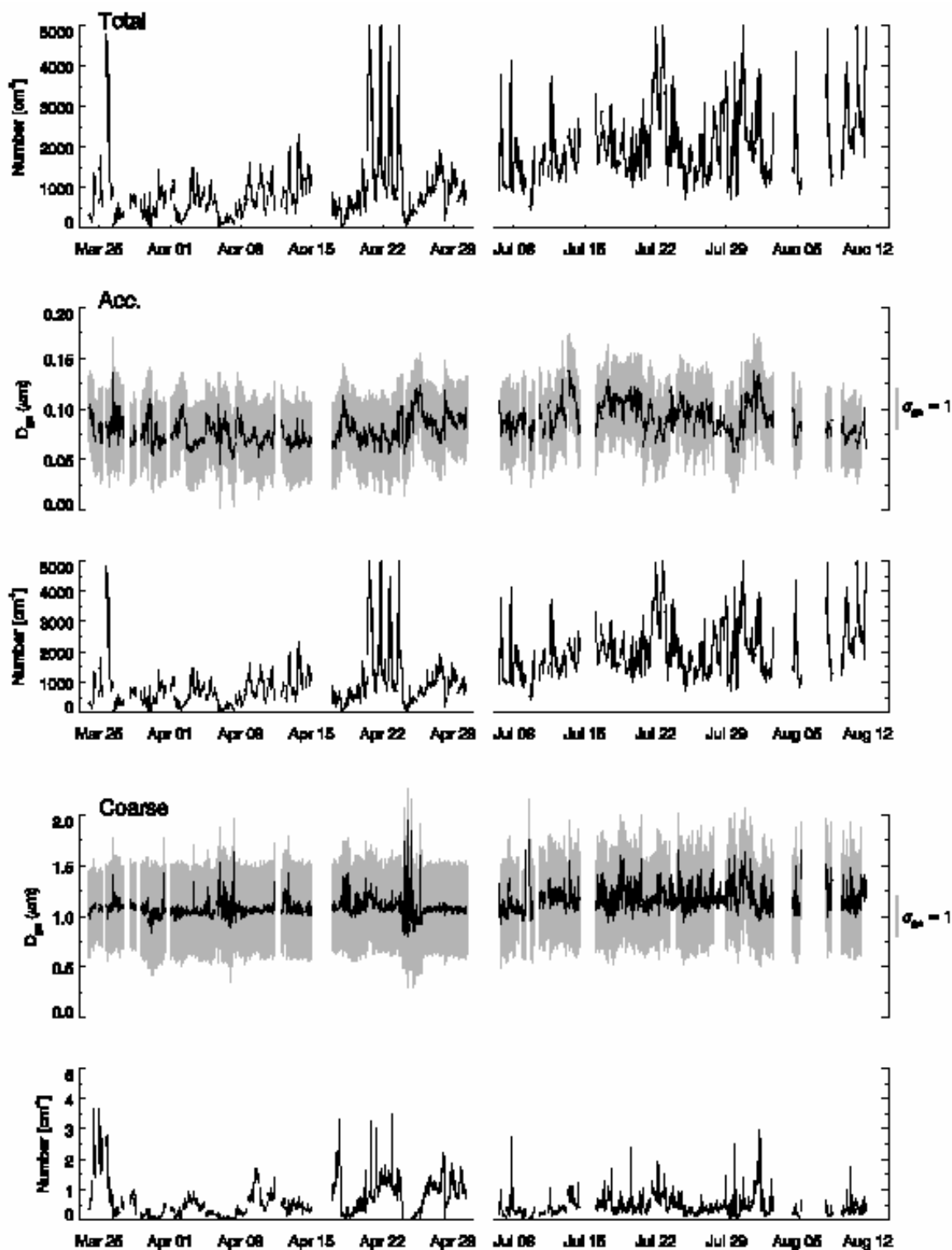
Figure 3.35. Integrated total (top), accumulation mode (middle), and coarse mode (bottom) aerosol number concentrations [ \text{cm}^{-3} ]. Top time series in the middle and bottom panels show mode geometric mean diameter ( \mu\text{m} , black line) and geometric standard deviation (right axis, gray shading).
