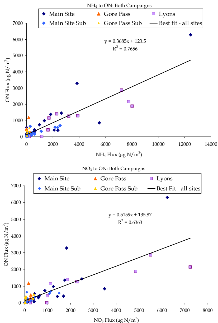
Figure 4.23. Relationship between organic and inorganic nitrogen wet deposition fluxes ( \mu\text{g}/\text{m}^2 ) during the RoMANS study. Data are included from the three locations where ON was measured: the core site, Lyons, and Gore Pass.
