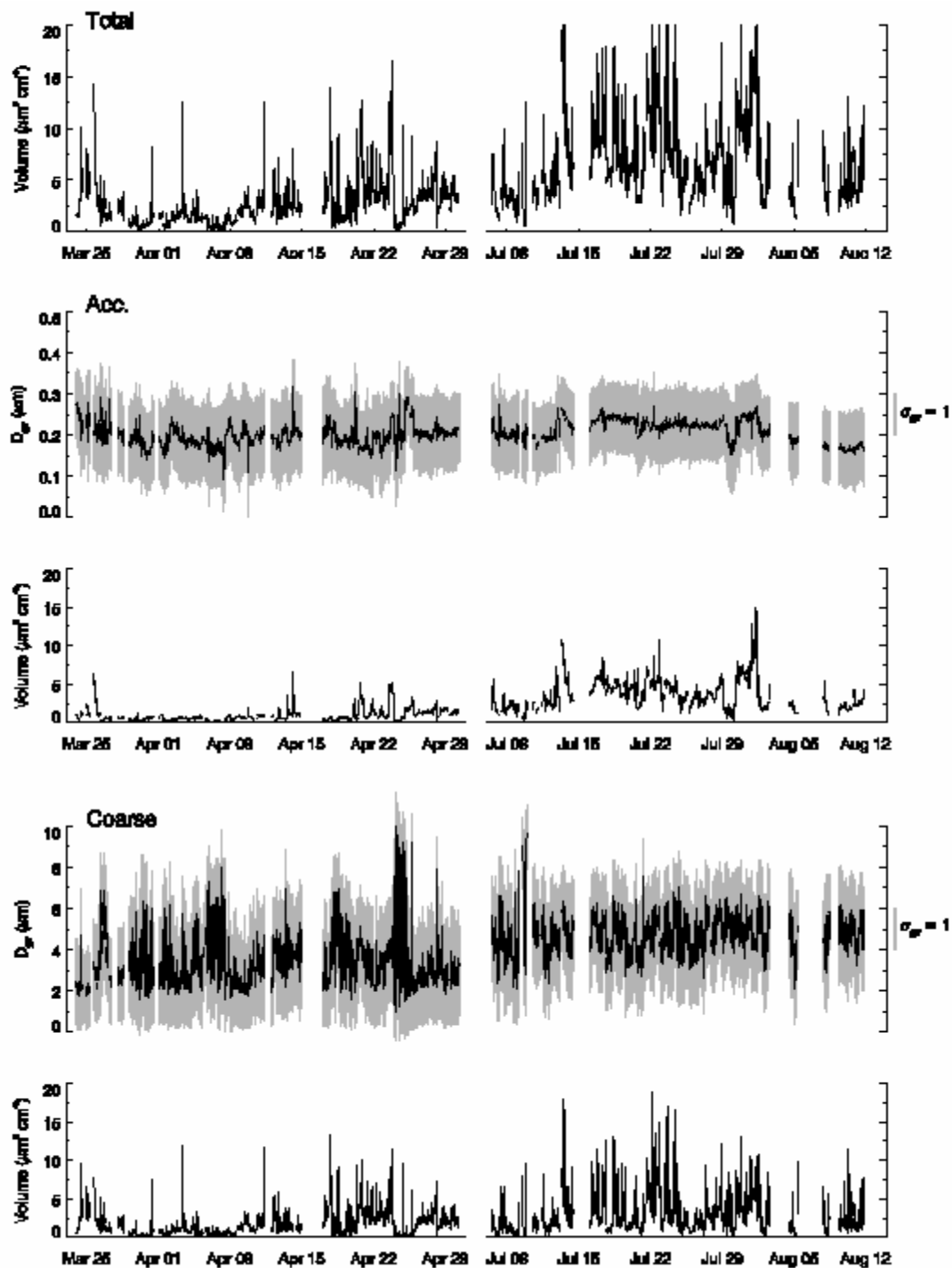
Figure 3.36. Integrated total (top), accumulation mode (middle), and coarse mode (bottom) aerosol volume concentrations [ \mu\text{m}^3 \text{cm}^{-3} ]. Top time series in the middle and bottom panels show mode geometric mean diameter ( \mu\text{m} , black line) and geometric standard deviation (right axis, gray shading).
