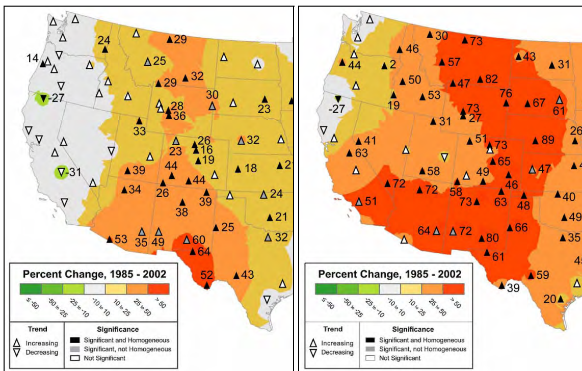
Figure S.2. Left panel: Percent changes in the nitrate concentrations in precipitation for the years 1985–2002. Right panel: Percent changes in the ammonium concentrations in precipitation for the years 1985–2002 (Lehmann et al., 2005, reproduced without permission).
