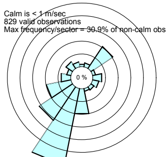
Estes Park Radar Profiler spring 97-m mode 4500-6000 m AGL
