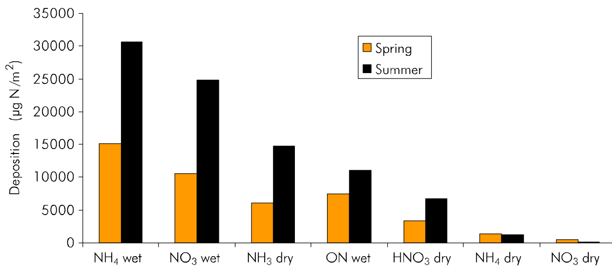
Figure 4.22. Nitrogen deposition totals ( \mu\text{g N/m}^2 ) by various species and pathways in order of contribution to total nitrogen deposition at the RoMANS core site.
