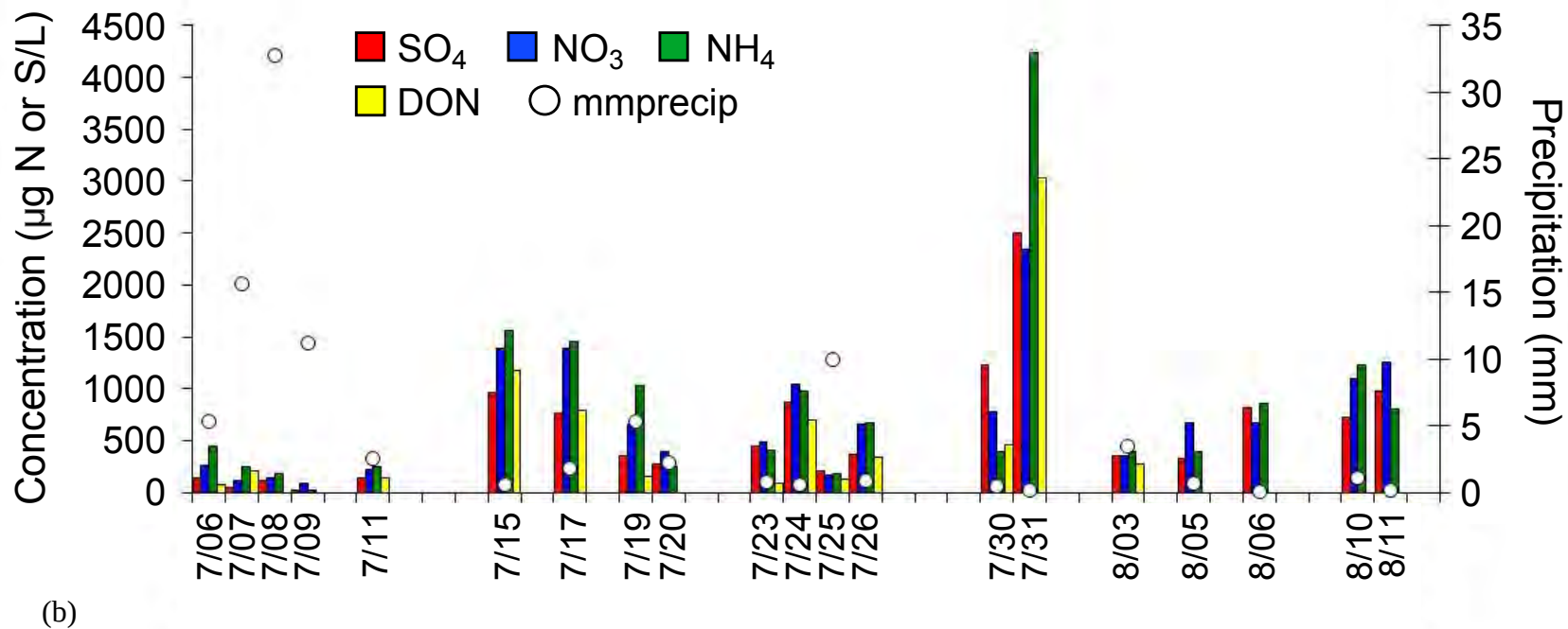
Figure 3.10. Time line of major species concentrations ( \mu\text{g/L} ) measured in precipitation collected at the RoMANS core site during the (a) spring and (b) summer field campaigns.
