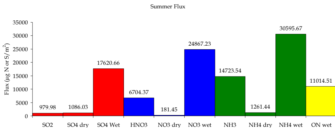
Figure 4.18. RoMANS core site summer deposition fluxes ( \mu\text{g}/\text{m}^2 ) broken down for each species by dry gaseous, dry particle, and wet.
