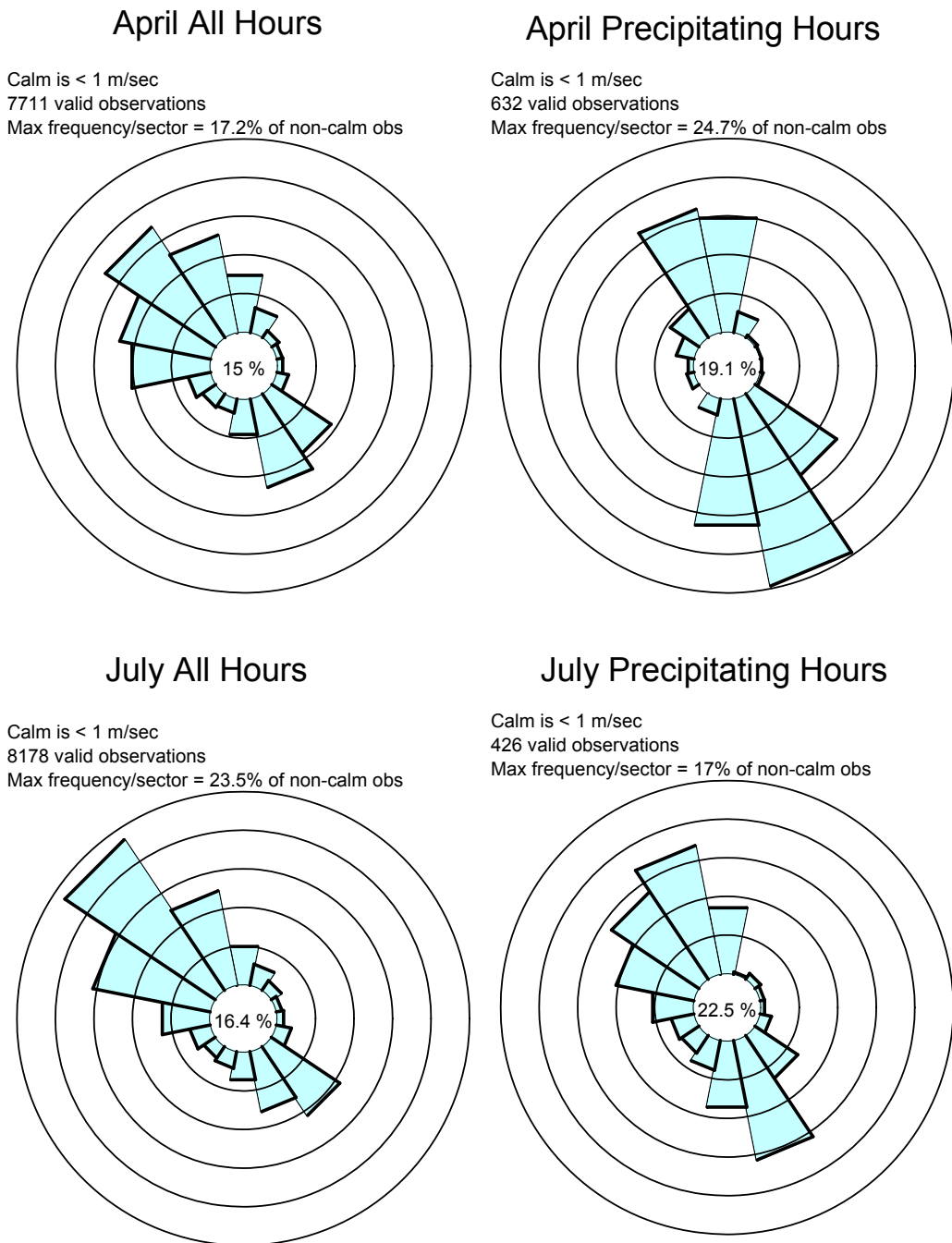
Figure 1.12. Directional frequencies of winds from 16 directional bins at the RoMANS core site during 1995–2005 for April (top) and July (bottom) for all hours (left) and hours with precipitation (right). Data are from the NPS gaseous monitoring network. Each ring is five percent.
