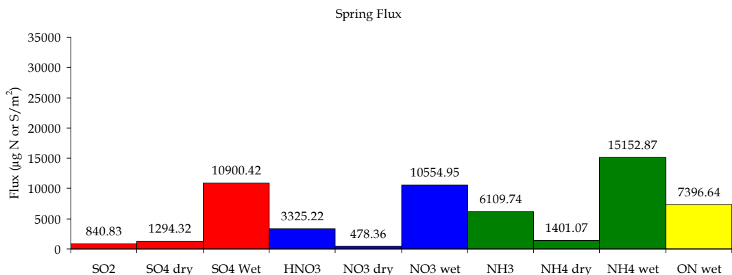
Figure 4.17. RoMANS core site spring deposition fluxes ( \mu\text{g}/\text{m}^2 ) broken down for each species by dry gaseous, dry particle, and wet.
